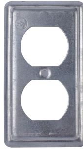
3301 Blank Galvanized Cover 4-3/32" x 2-7/32" 200 pcs in a carton
