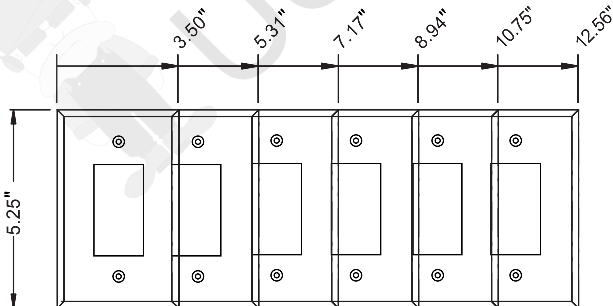
1-6 Gang Over-size Dimensions
