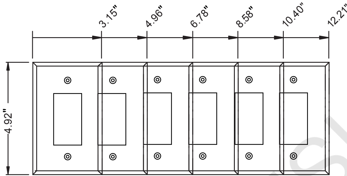
1-6 Gang Mid-size Dimensions
